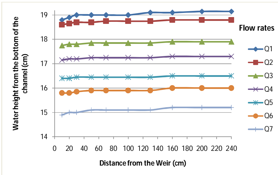
Figure 2: Water Surface Profile for Different Discharges
